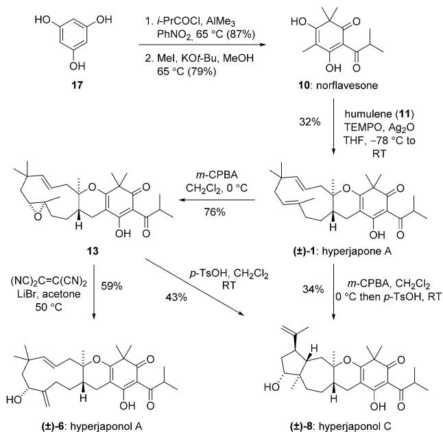
Scheme 2. Total synthesis of hyperjapone A and hyperjaponols A and C. TEMPO = (2,2,6,6-tetramethylpiperidin-1-yl)oxyl; m -CPBA = 3-chloroperoxy-benzoic acid; p -TsOH = p -toluenesulfonic acid.
