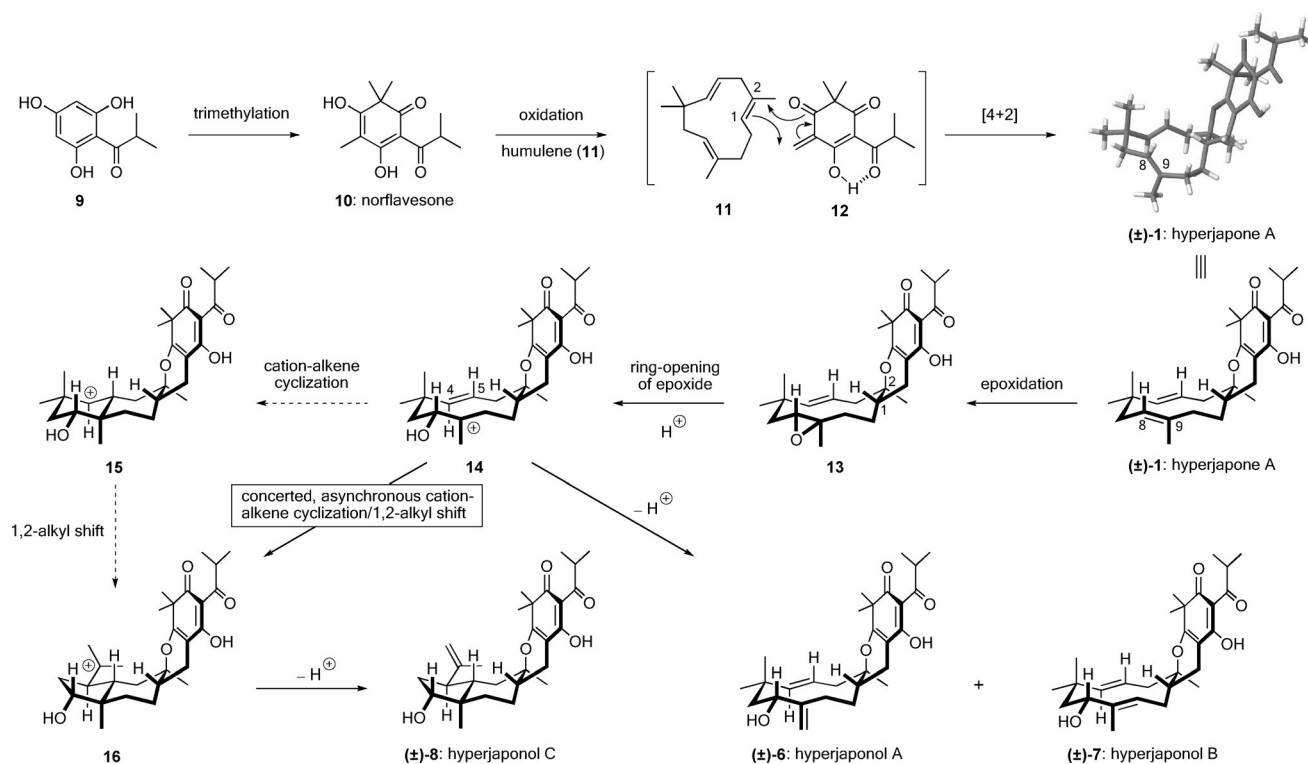
Scheme 1. Proposed biosynthesis of hyperjaponol C from hyperjapone A through a concerted, asynchronous alkene cyclization/1,2-alkyl shift.
